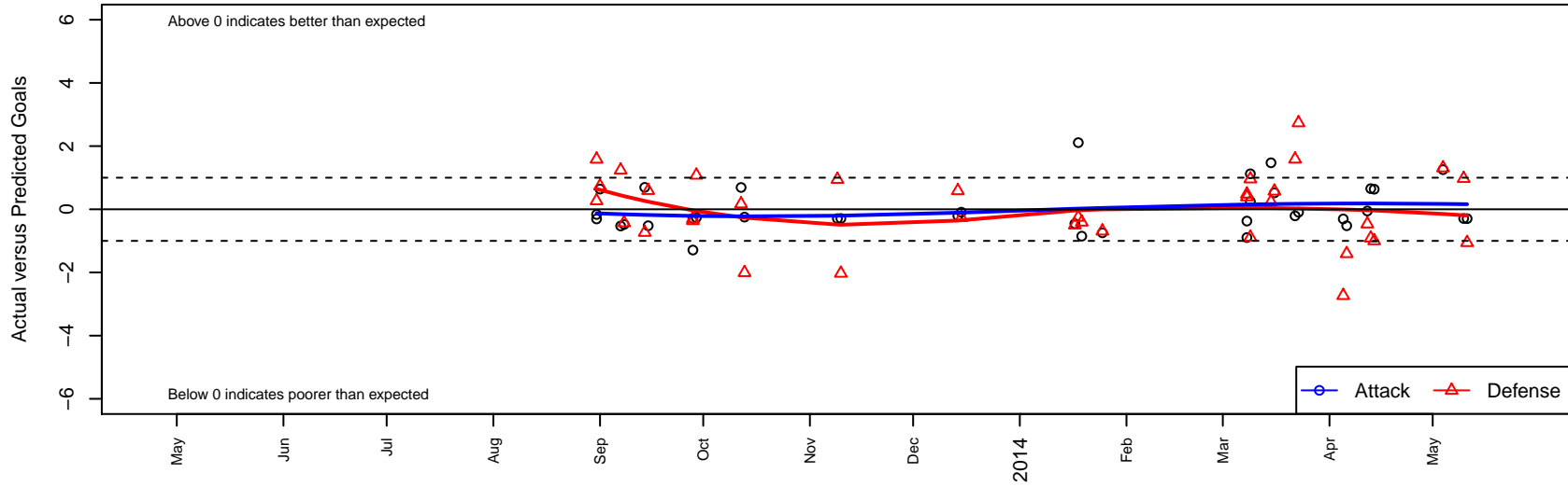
Heat FC ECNL G99 Dots are actual minus expected GF (blue circles) and GA (red triangles). Blue line is smoothed change in attack strength. Red is smoothed change in defense strength.
